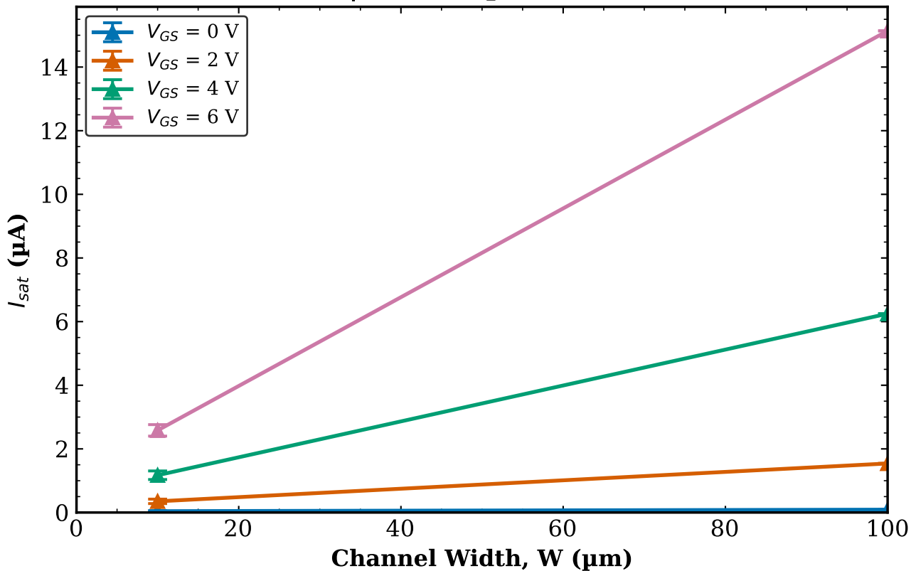
TFT3 Combined (Tr. 1 & 2) I_{sat} vs W | L = 80\text{ }\mu\text{m} (mean \pm std)
